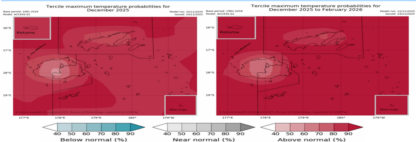
Figure 5: Maximum Air Temperature Predictions: December & December 2025 to February 2026
