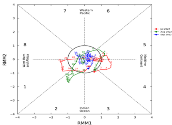
(RMM1, RMM2) phase space for 01-Jul-2022 to 30-Sep-2022
