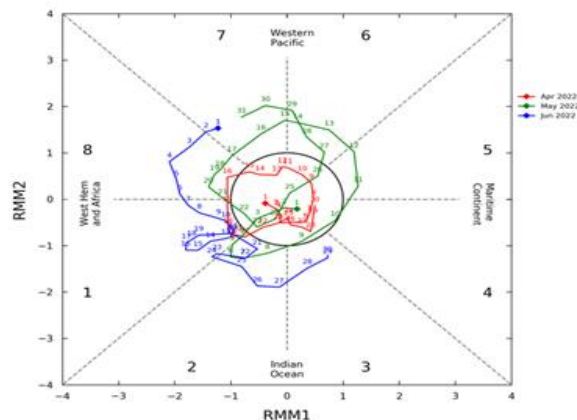
(RMM1, RMM2) phase space for 01-Apr-2022 to 30-Jun-2022
